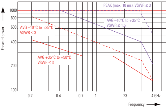
Power-handling capacity
