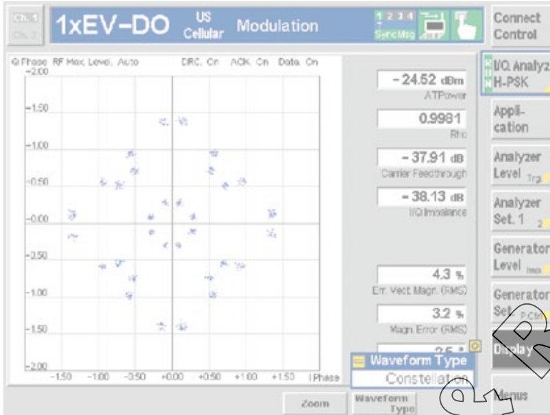
The I/Q analyzer provides a constellation diagram as well as an eye pattern for the Land Q component.
