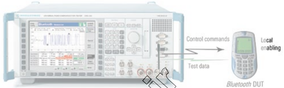
The DUT can be connected to the R&S® CMU 200 via an RF coupler (antenna) or a cable.
