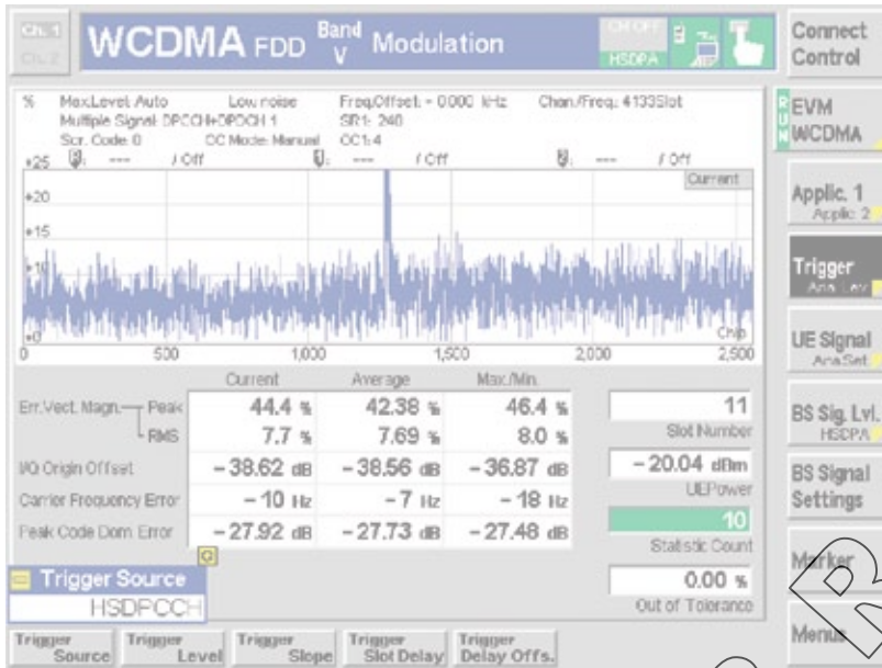
This screenshot shows the effect of a power rise after the first five SF256 symbols in the slot. An EVM, magnitude and phase error surge appears. The HS-DPCCH trigger in the case of the modulation measurements always marks the DPCCH slot that contains the start of an HS-DPCCH subframe in which a valid ACK or NACK is expected.
