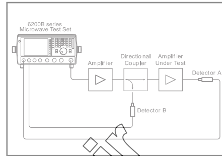
Test Set up for Rated Measurements
