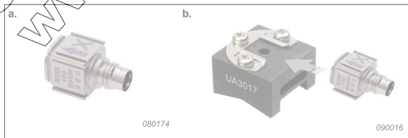
Fig. 4 a. Triaxial accelerometer Type 4524-B-001 b. Mounting Type 4524-B-001 in the clip on mounting adaptor UA-3017
